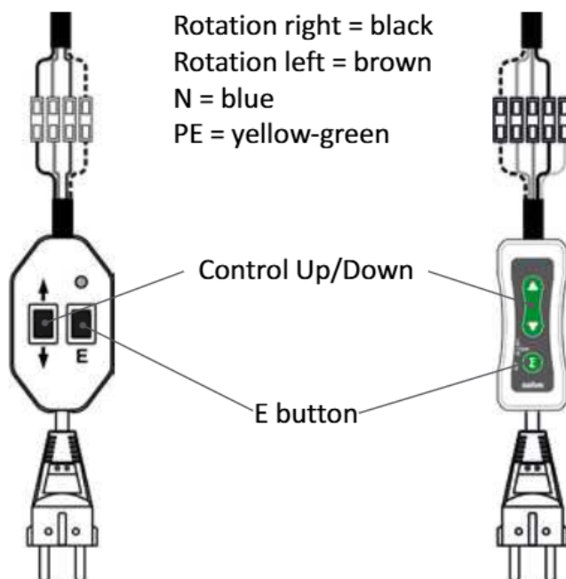
SELVE setting switch article no. 290103
