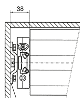
Wandanker 13 106.3501
