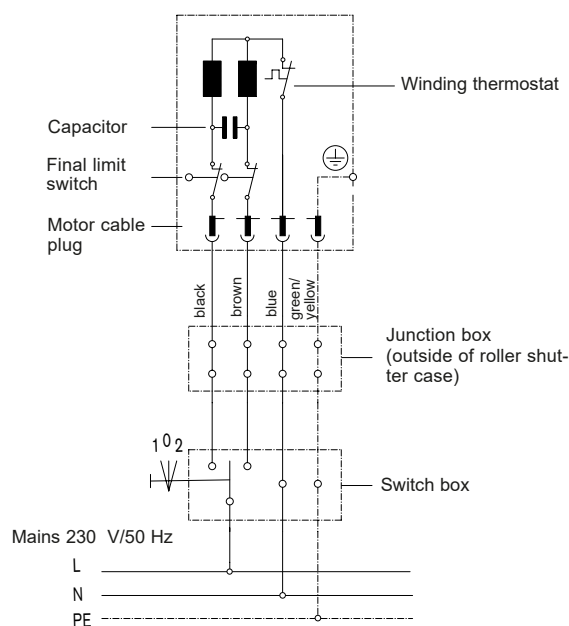
Fig. 4 Circuit diagram VariEco with 230 V / 50 Hz
